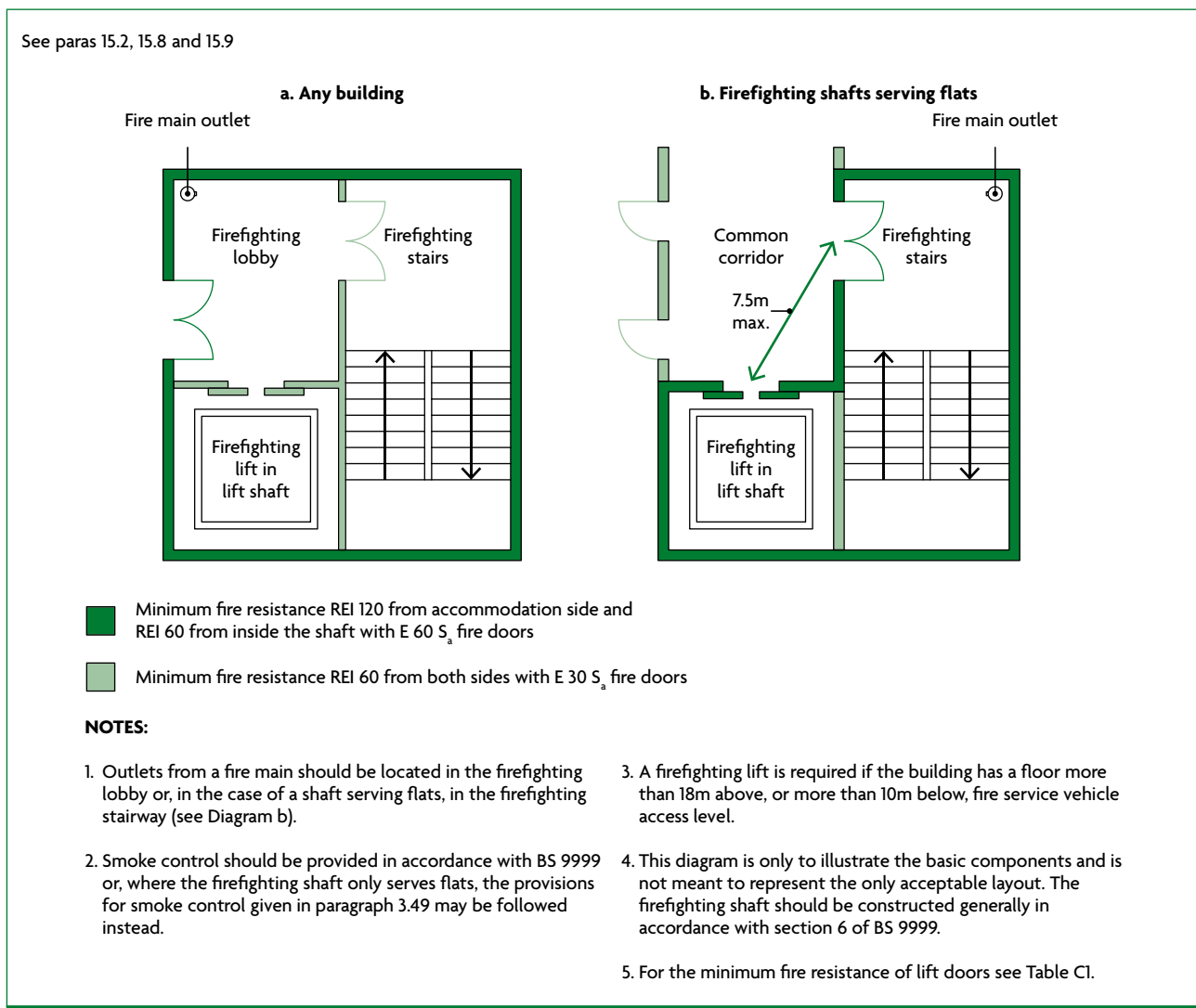
Diagram 15.1 Components of a firefighting shaft
